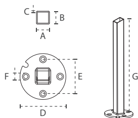
ROUND SUPPORT
