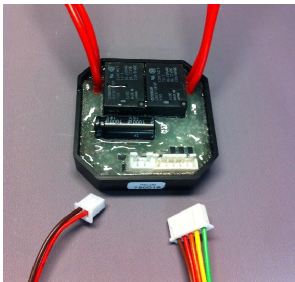
Figure 1 : module relais REL02
