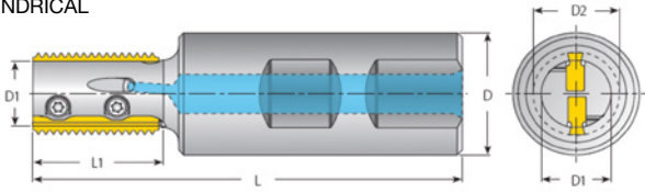
CYLINDRICAL
