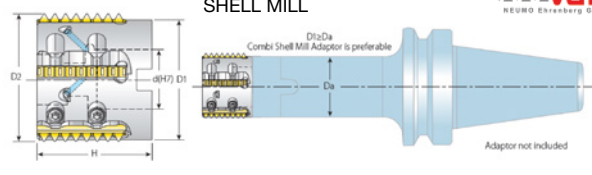
SHELL MILL
