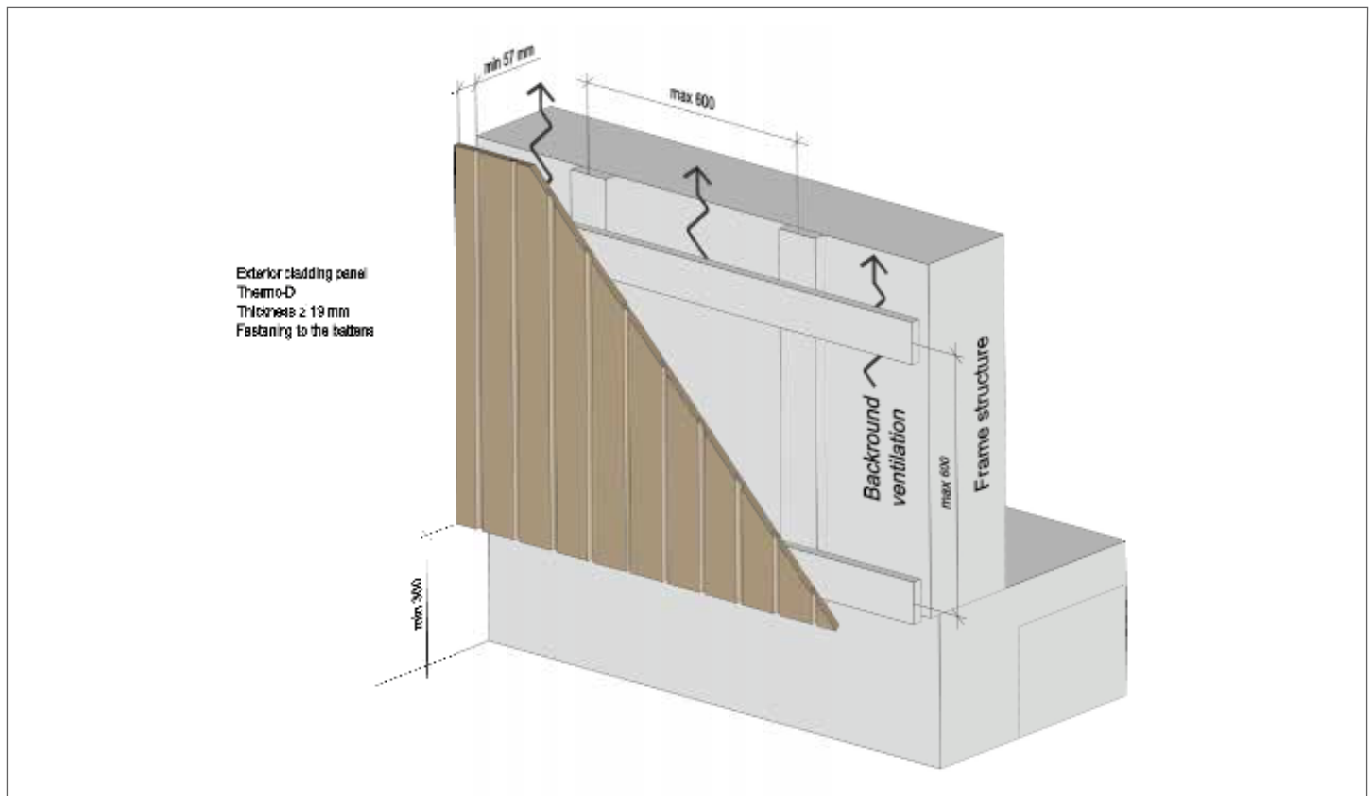
Figure 46. An example of exterior wall cladding.
