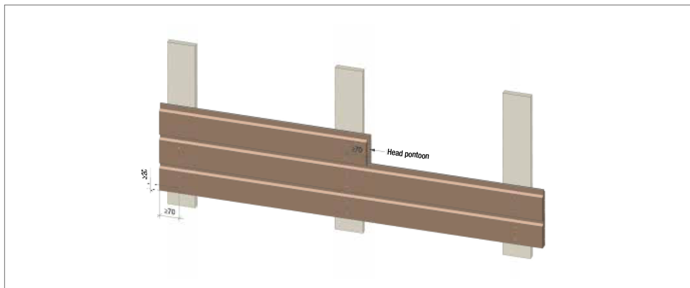
Figure 52. The recommended distances to edges and ends without pre-drilling with ThermoWood® products.
