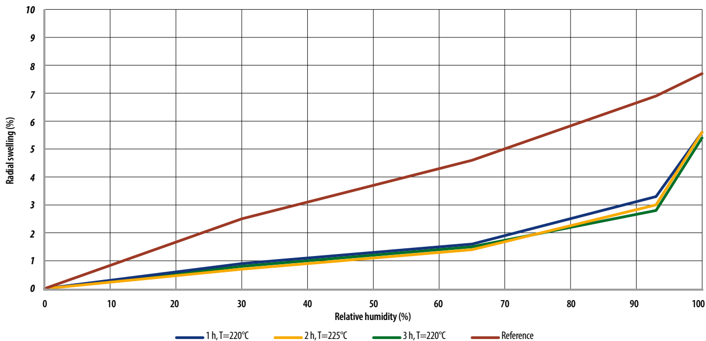
Figure 28. Radial swelling of spruce as a function of relative humidity (source: VTT).
