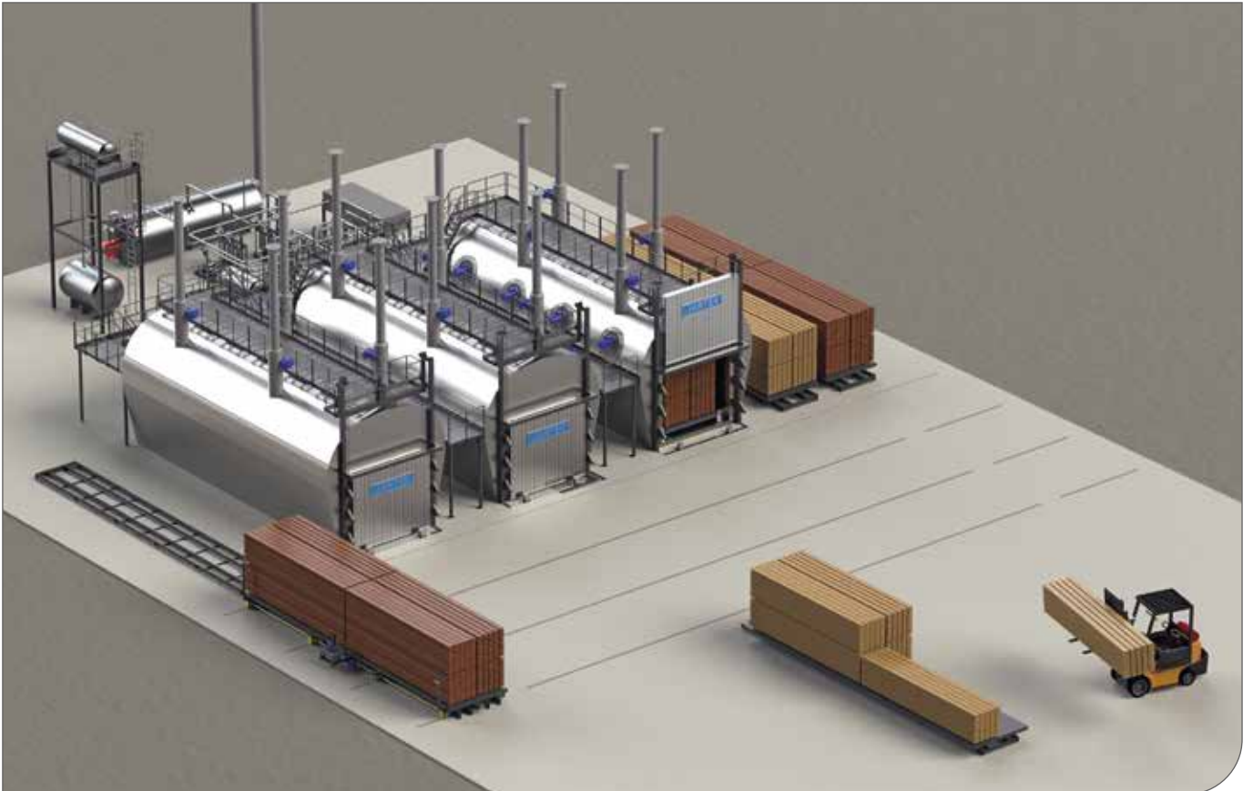
Figure 7. ThermoWood® plant.
