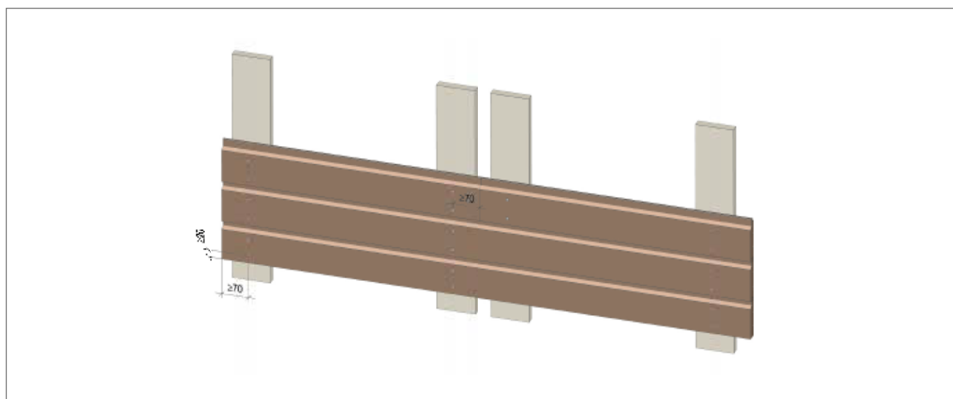
Figure 53. The recommended distances to edges and ends without pre-drilling with ThermoWood® products (without tongue and groove joint).
