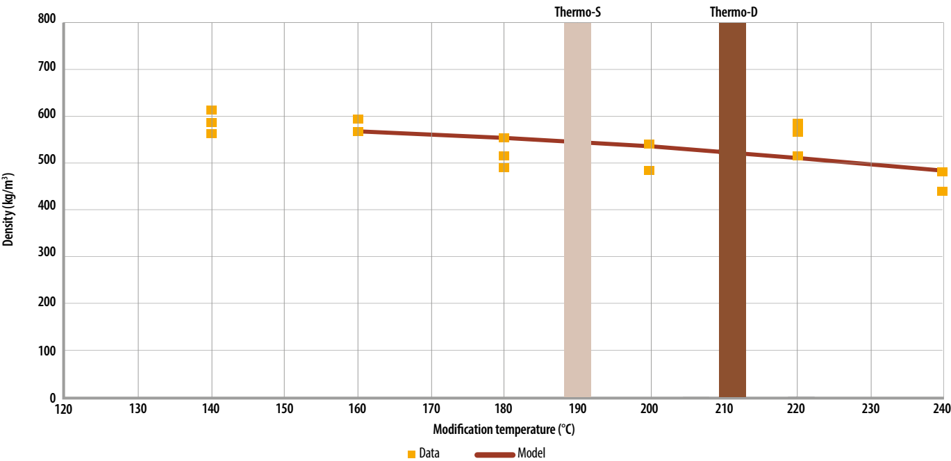
Figure 22. The impact of the modification temperature on the density of ThermoWood® (source: VTT).
