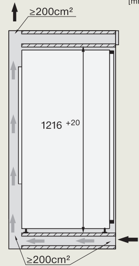
K 7347 C, K 7348 C, K 7377 B, K 7378 B
