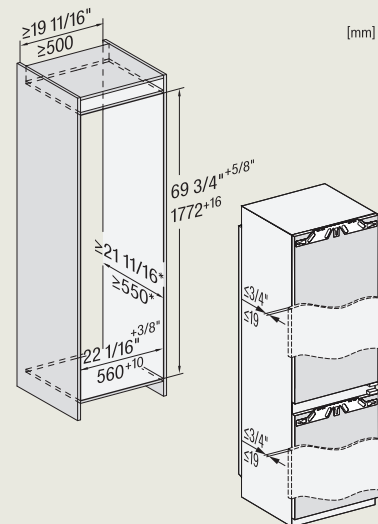
KFN 7795 C
