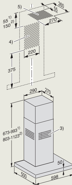
DAW 1620 Active wanddampkap
